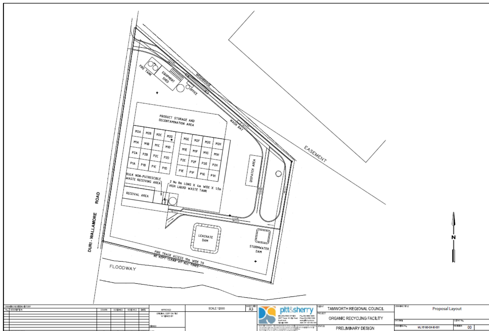
Figure 3 Proposed Facility Layout
