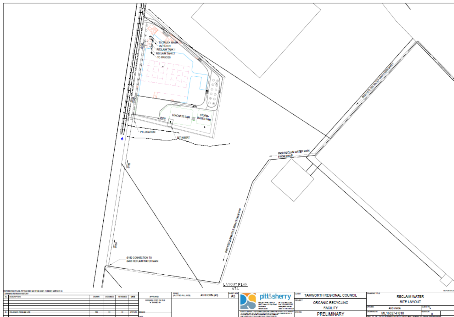
Figure 5 Ancillary Pipeline Works Plan
