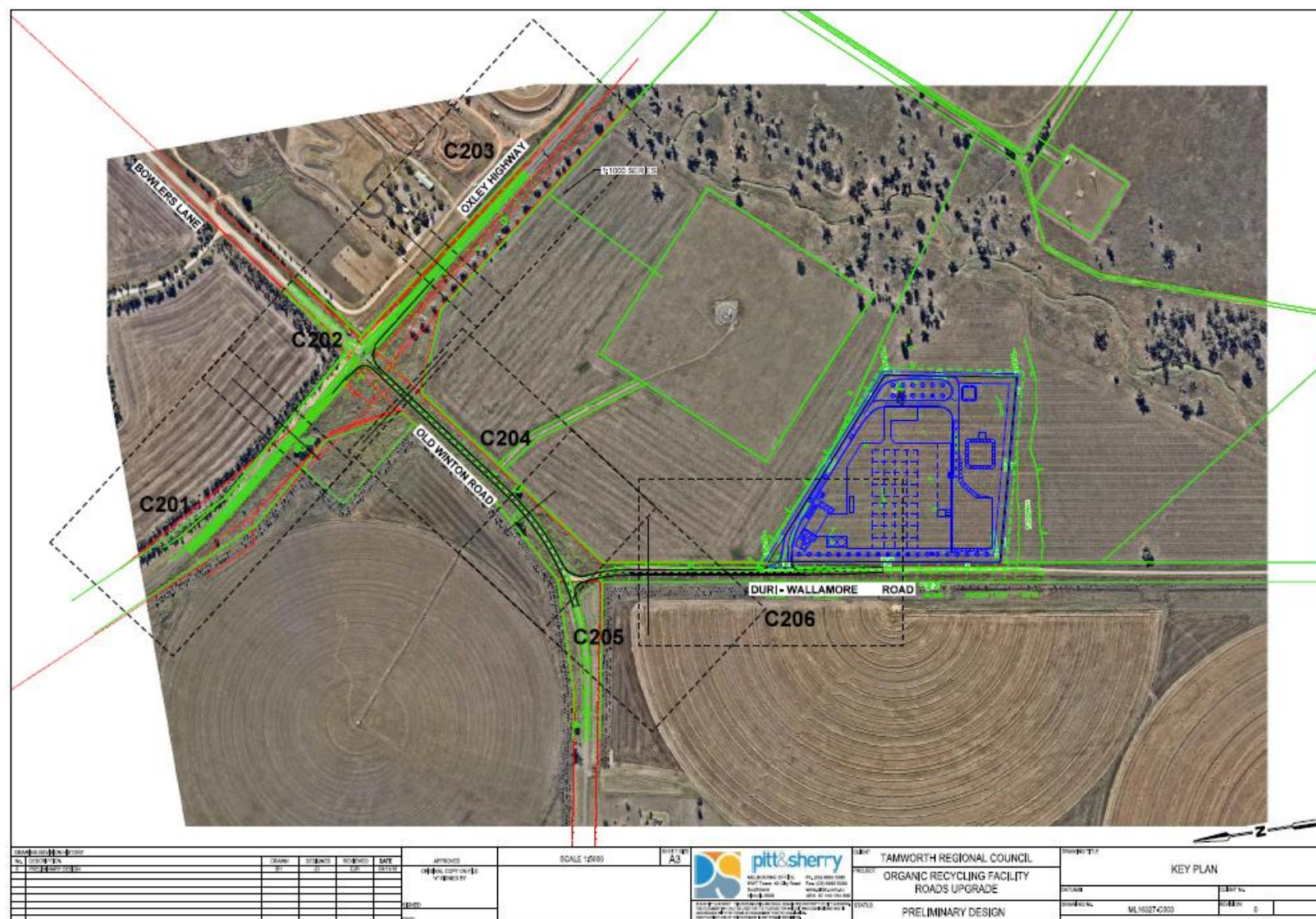
Figure 4 Ancillary Road Works Plan
